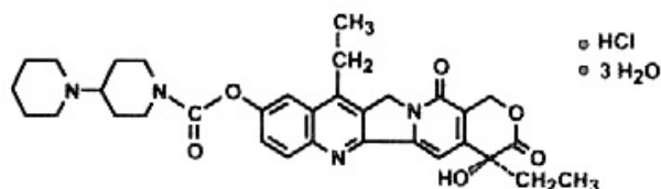
Irinotecan Hydrochloride
