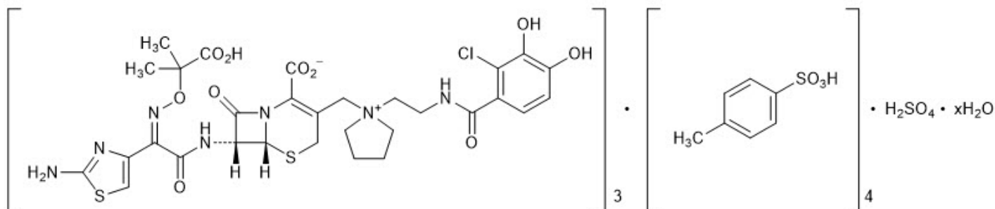
Figure 1 Chemical Structure of Cefiderocol Sulfate Tosylate
