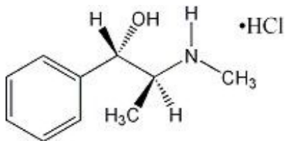
Pseudoephedrine Hydrochloride Structure Image
