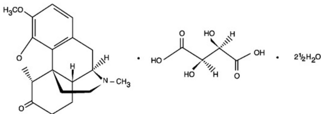
Hydrocodone Bitartrate
