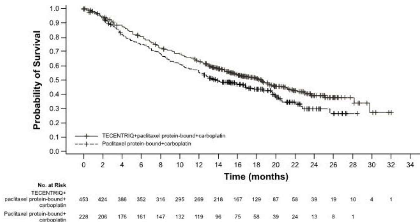
Figure 4: Kaplan-Meier Curves for Overall Survival in IMpower130
