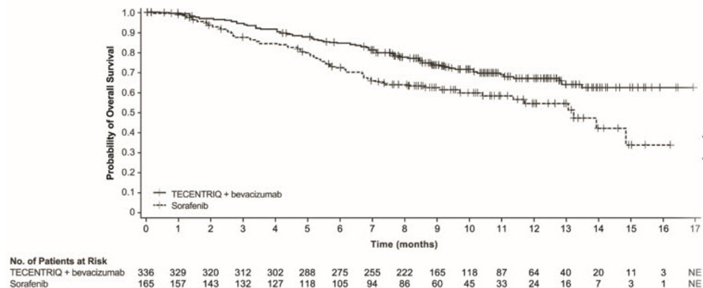
Figure 7: Kaplan-Meier Plot of Overall Survival in IMbrave150
