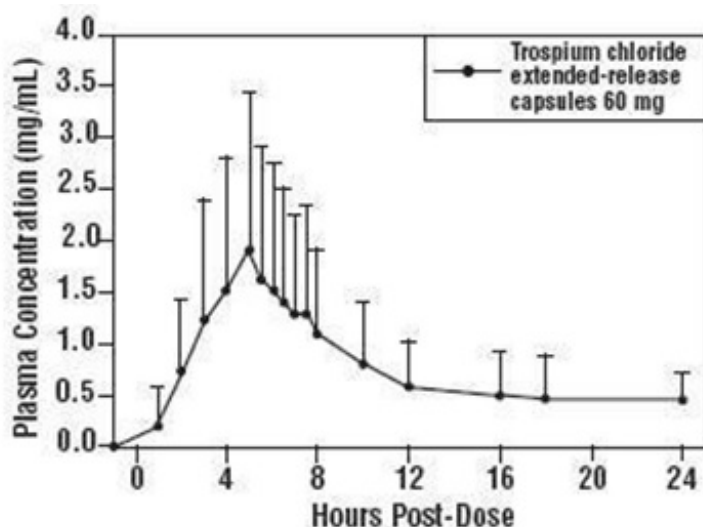
Figure 1: Mean (+SD) Concentration- Time Profile for a Single 60 mg Oral Dose of Trospium Chloride Extended- Release Capsules in Healthy Volunteers
