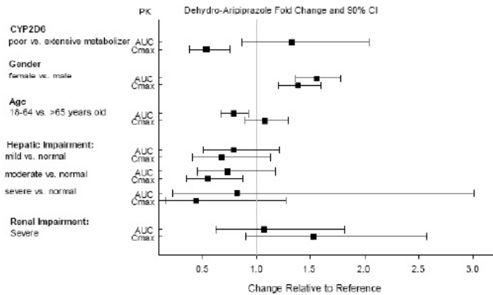
Figure 5: Effects of intrinsic factors on dehydro-aripiprazole pharmacokinetics
