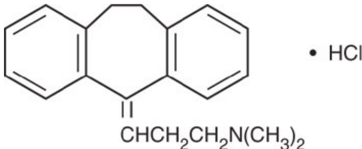
AMITRIPTYLINE 75MG STRUCTURE
