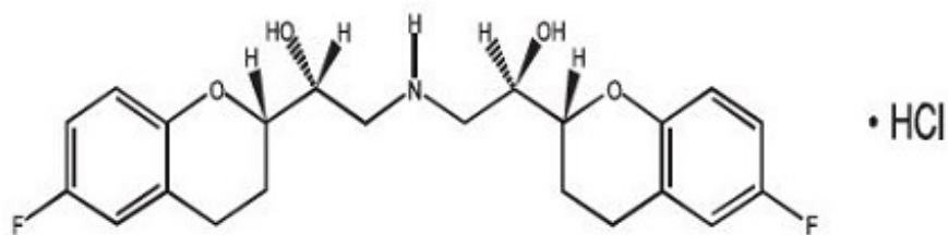
SRRR - or d-nebivolol hydrochloride
