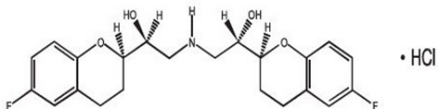
RSSS - or l-nebivolol hydrochloride
