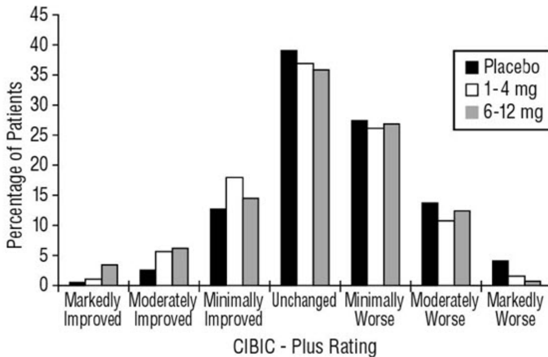
Figure 3 Frequency Distribution of CIBIC-Plus Scores at Week 26 in Study 1
