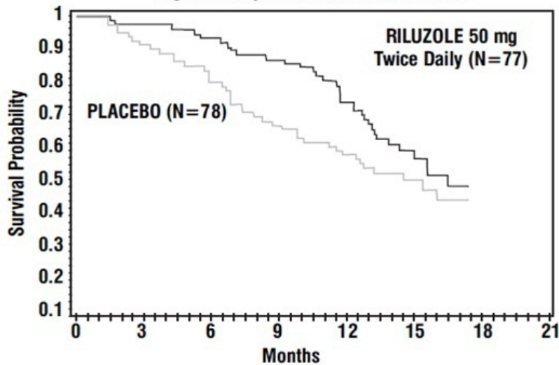
Figure 1: Kaplan-Meier Survival Curves
