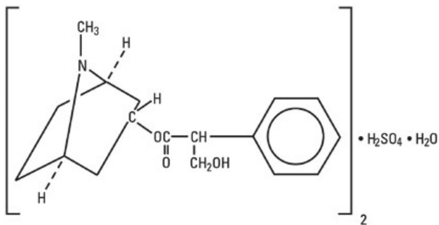
Atropine Sulfate Structural Formula
