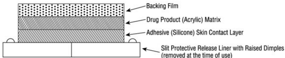
Figure 1: Cross Section of the Rivastigmine Transdermal System
