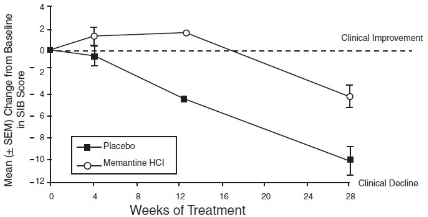
Figure 3: Time course of the change from baseline in SIB score for patients completing 28 weeks of treatment.
