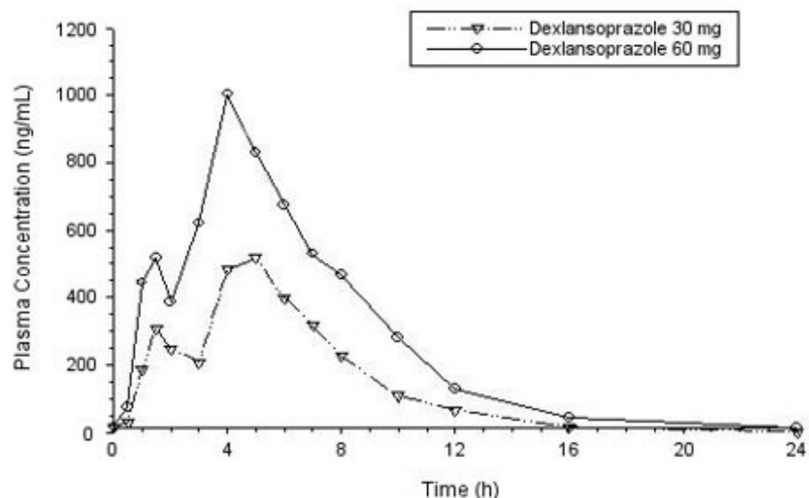
Figure 1: Mean Plasma Dexlansoprazole Concentration - Time Profile Following Oral Administration of 30 or 60 mg Dexlansoprazole Once Daily for 5 Days in Healthy Adult Subjects
