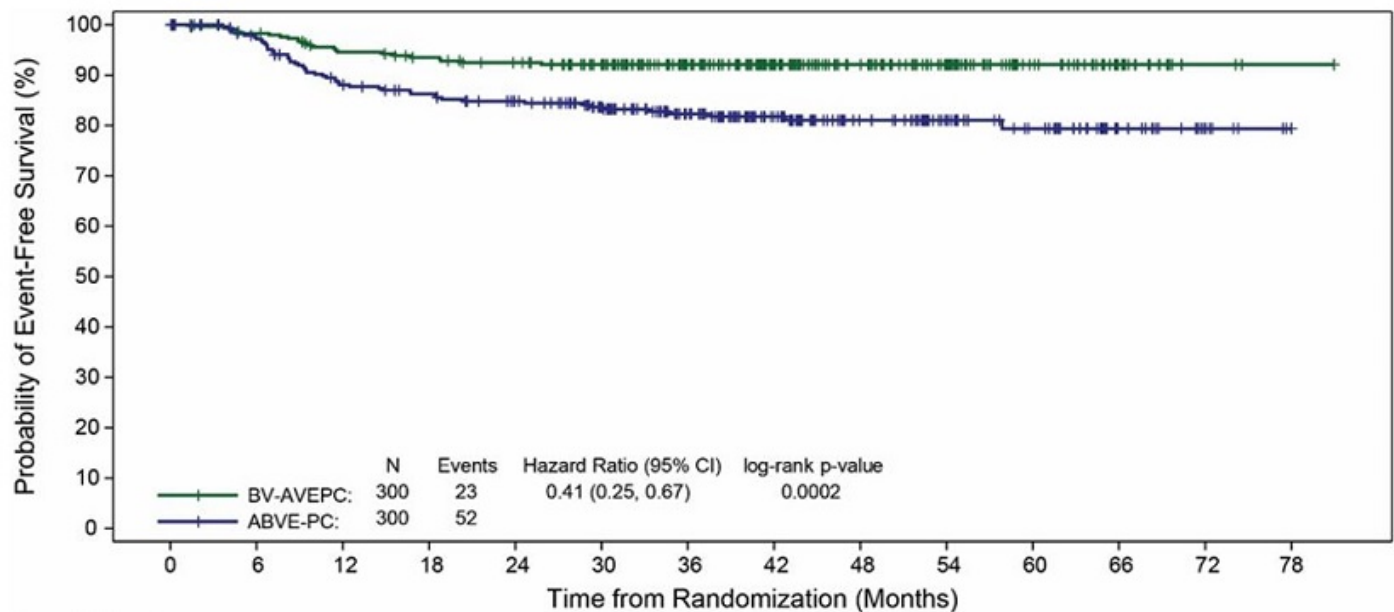
Figure 3: Kaplan-Meier Curve of Event-Free Survival (Study 7: AHOD1331)
