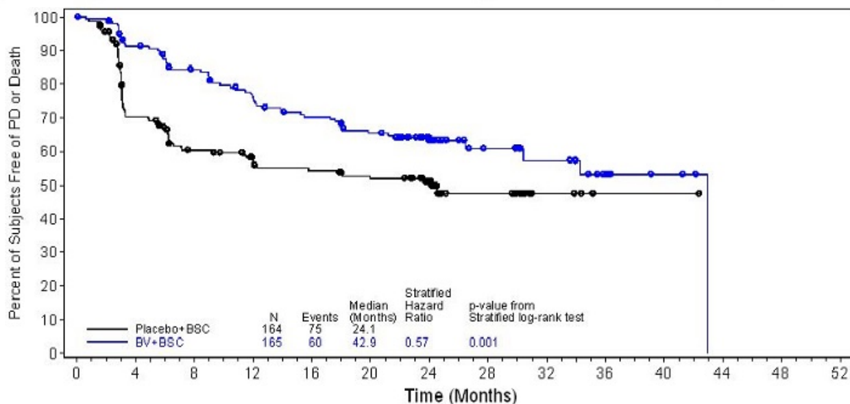
Figure 4: Kaplan-Meier Curve of IRF-Assessed Progression-Free Survival (Study 3: AETHERA)
