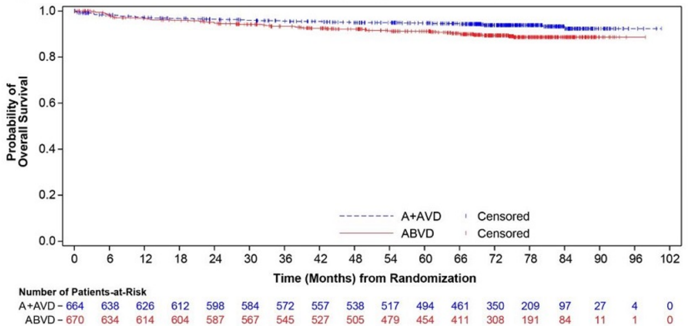
Figure 2: Kaplan-Meier Curve of Overall Survival (Study 5: ECHELON 1)
