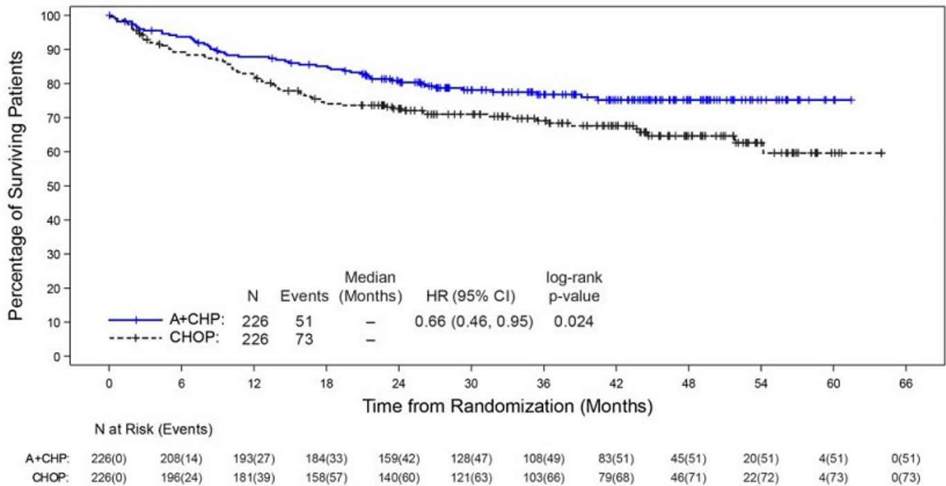
Figure 6: Kaplan-Meier Curve of Overall Survival (Study 6: ECHELON-2)
