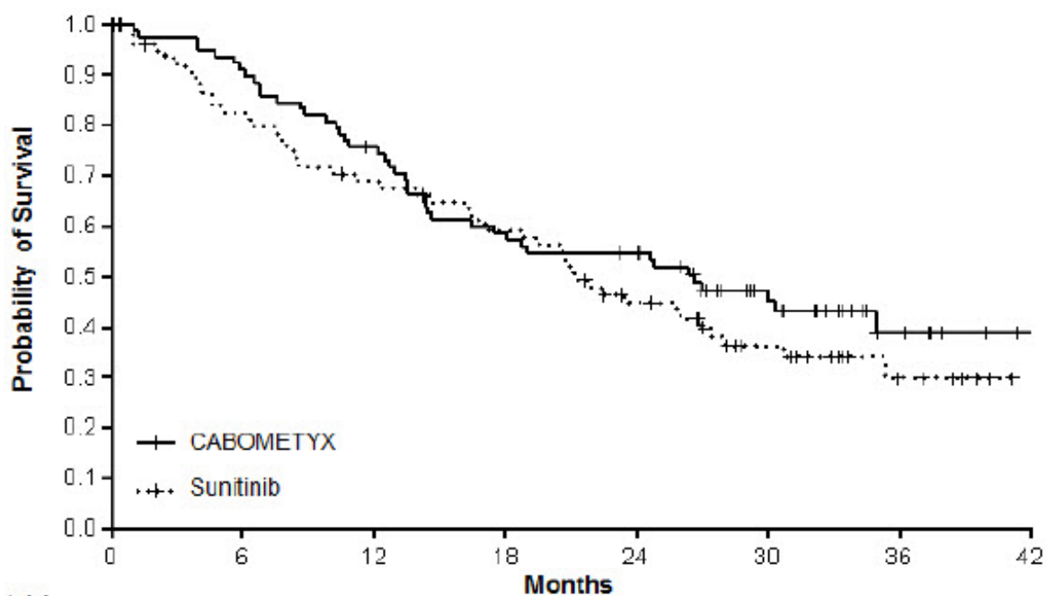
Figure 4: Kaplan-Meier Curve of Overall Survival in CABOSUN
