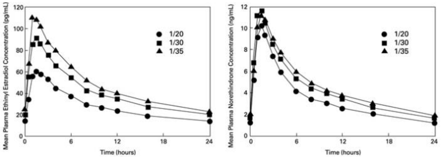
Figure 1. Mean Steady-State Plasma Ethinyl Estradiol and Norethindrone Concentrations Following Chronic Administration of TILIA Fe
