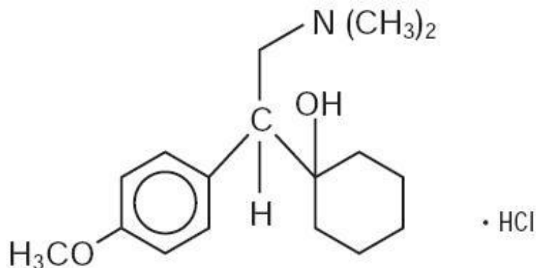
Venlafaxine hydrochloride
