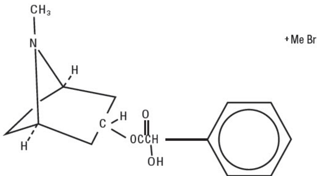
C 17 H 24 BrNO 3 HOMATROPINE METHYLBROMIDE
