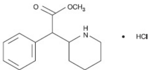
Methylphenidate Hydrochloride
