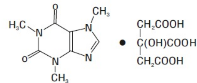
Caffeine citrate C_{14}H_{18}N_4O_9 Mol. Wt. 386.31
