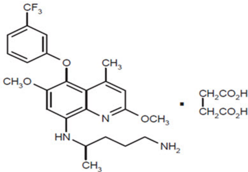
Figure 1: Tafenoquine Succinate Structure
