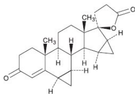
Drospirenone
