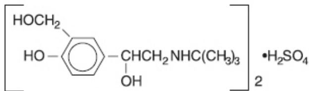
Figure 3.1-1. Chemical structure of albuterol sulfate.
