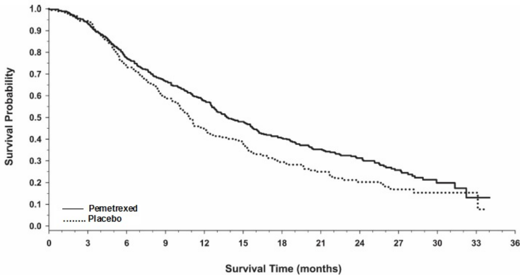
Figure 8: Kaplan-Meier Curves for Overall Survival in PARAMOUNT
