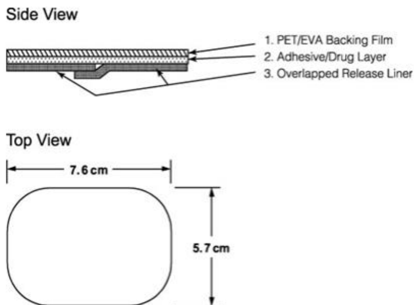
Figure 1: Side and top views of the OXYTROL transdermal system. (Not to scale)
