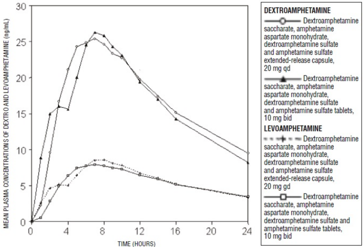
Figure 1 Mean d-amphetamine and l-amphetamine Plasma Concentrations Following Administration of dextroamphetamine saccharate, amphetamine aspartate monohydrate, dextroamphetamine sulfate and amphetamine sulfate extended-release capsules 20 mg (8 am) and dextroamphetamine saccharate, amphetamine aspartate monohydrate, dextroamphetamine sulfate and amphetamine sulfate tablets (immediate-release) 10 mg Twice Daily (8 am and 12 noon) in the Fed State.
