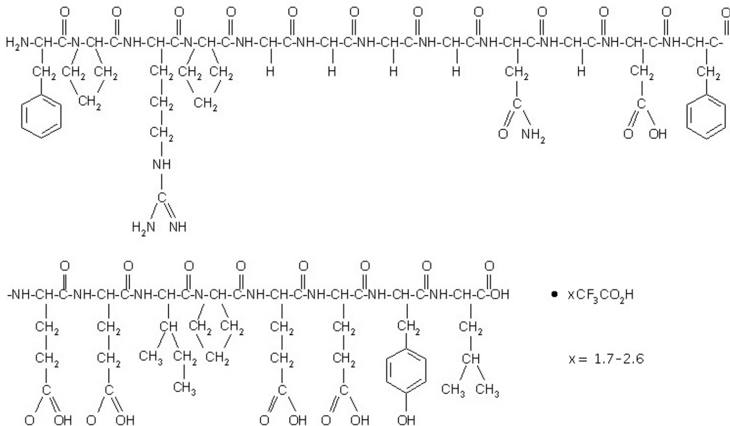
Figure 1: Structure Formula for Bivalirudin Trifluoroacetate
