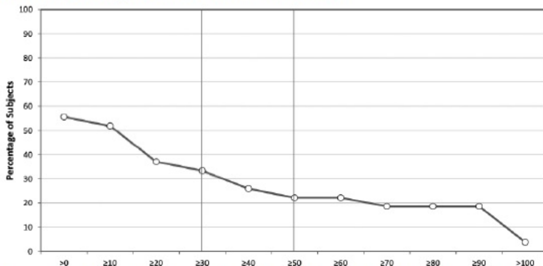
Figure 1: Percent Reduction Profiles for E_{max} of Drug Liking VAS for OXYCODONE HCl EXTENDED-RELEASE TABLETS vs. oxycodone HCl, N=27 Following Intranasal Administration
