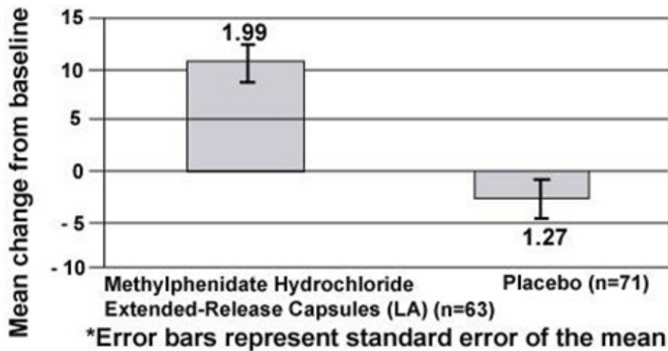
Figure 2. CADS- T Total Subscale - Mean Change from Baseline*
