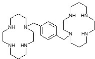
Figure 1: Structural Formula
