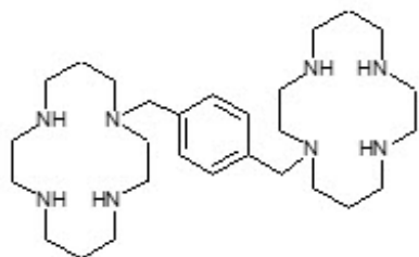
Figure 1: Structural Formula
