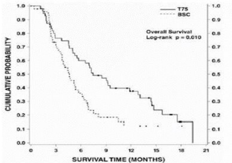
Figure 4 - TAX320 Survival K-M Curves - Docetaxel 75 mg/m 2 versus Vinorelbine or Ifosfamide Control
