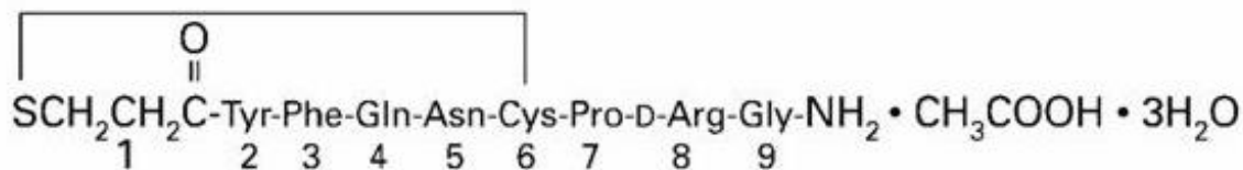
Structural Formula
