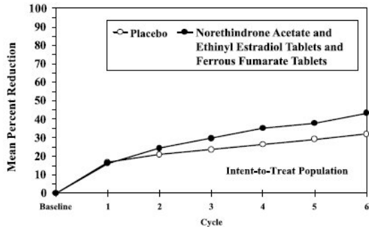
Figure 2. Mean Percent Reduction in Total Lesion Counts From Baseline to Each 28-Day Cycle and Mean Total Lesion Counts at Each Cycle Following Administration of Norethindrone acetate and ethinyl estradiol tablets and ferrous fumarate tablets and Placebo (Statistically significant differences were not found in both studies individually until cycle 6)
