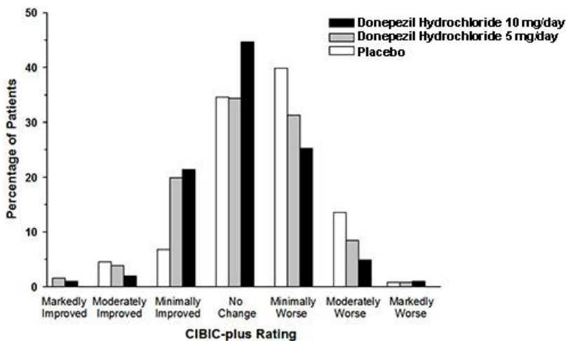
Figure 3. Frequency Distribution of CIBIC-plus Scores at Week 24.
