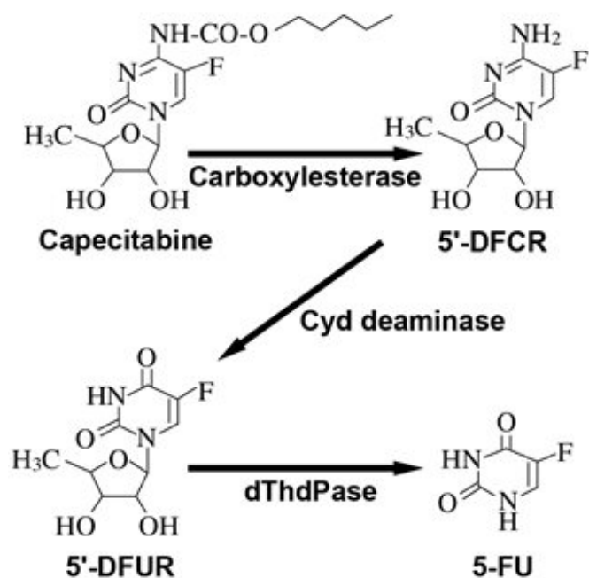
Metabolic Pathway of Capecitabine to 5-FU
