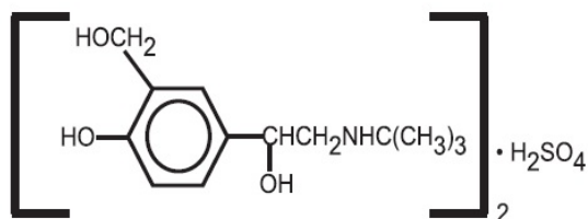
chemical structure of albuterol sulfate
