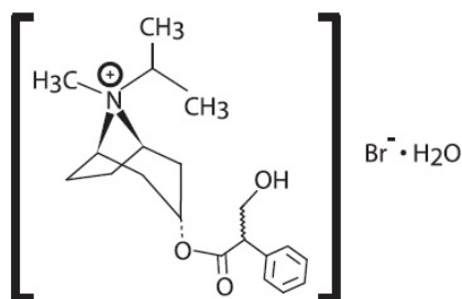
chemical structure of ipratropium bromide
