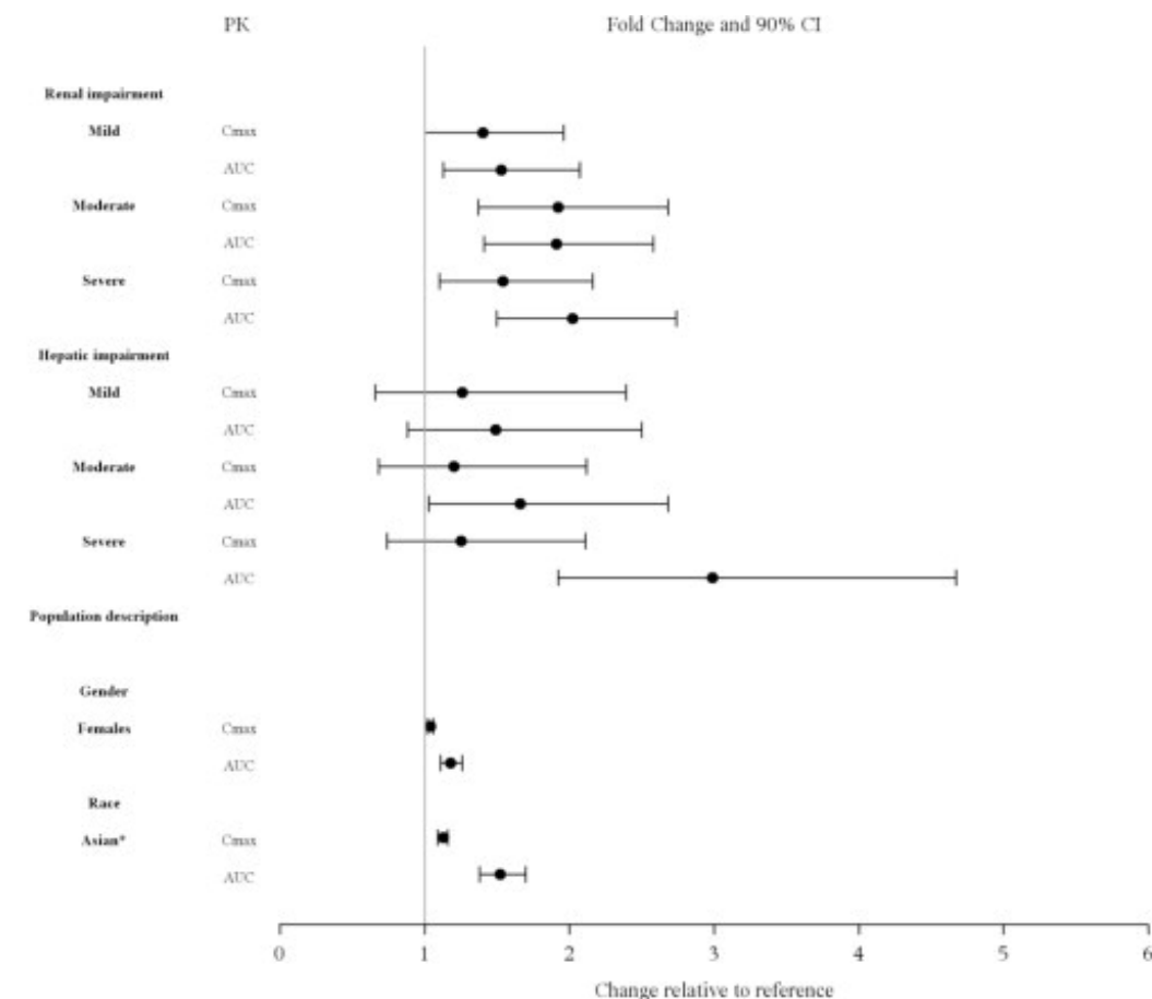
Figure 3: Impact of Other Patient Factors on LATUDA Pharmacokinetics
