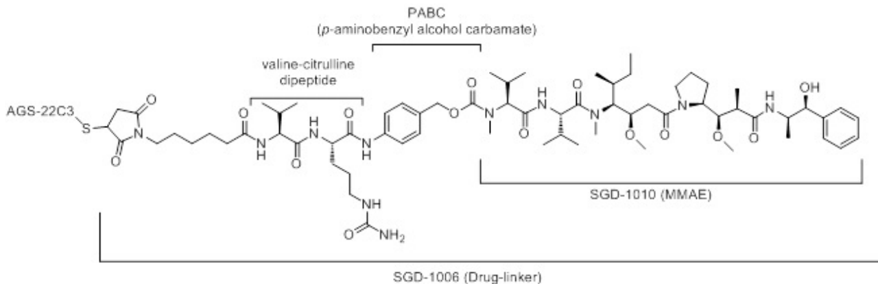
Figure 1. Structural Formula
